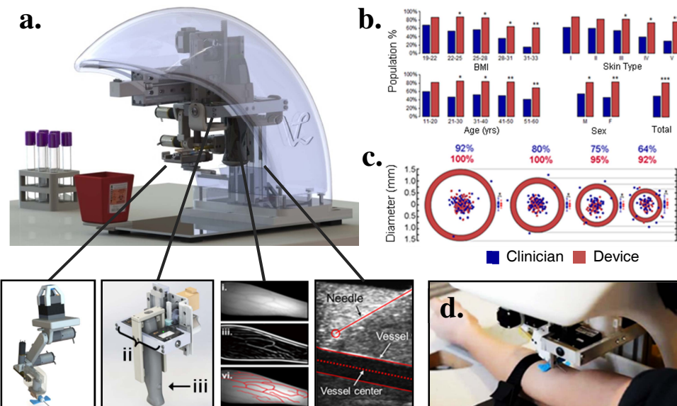
Figure 1. (a) Top: Computer render of device subsystems. Bottom: i, 4 DOF articulated manipulator arm; ii, near IR imaging system; iii, portable ultrasound system; iv, vein image segmentation; v, B-mode needle, vein, and blood flow detection. (b) Improved vein detection in 101 patients compared to a phlebotomist. (c) Improved accuracy on 288 customized tissue phantoms compared to a phlebotomist. (d) IRB-approved first-in-human device testing initiated at Rutgers University.
