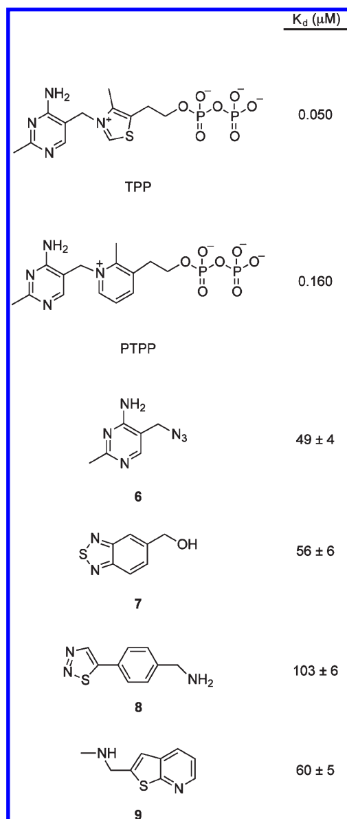
FIGURE 6. The TPP analog PTPP and select fragments that bind the TPP riboswitch: 5-(azidomethyl)-2-methylpyrimidin-4-amine ( 6 ), benzo[ c ]-[1,2,5]thiadiazol-5-ylmethanol ( 7 ), (4-(1,2,3-thiadiazol-5-yl)phenyl)methanamine ( 8 ), and N -methyl-1-(thieno[2,3- b ]pyridin-2-yl)methanamine ( 9 ). K_D values from refs 35 and 61.
