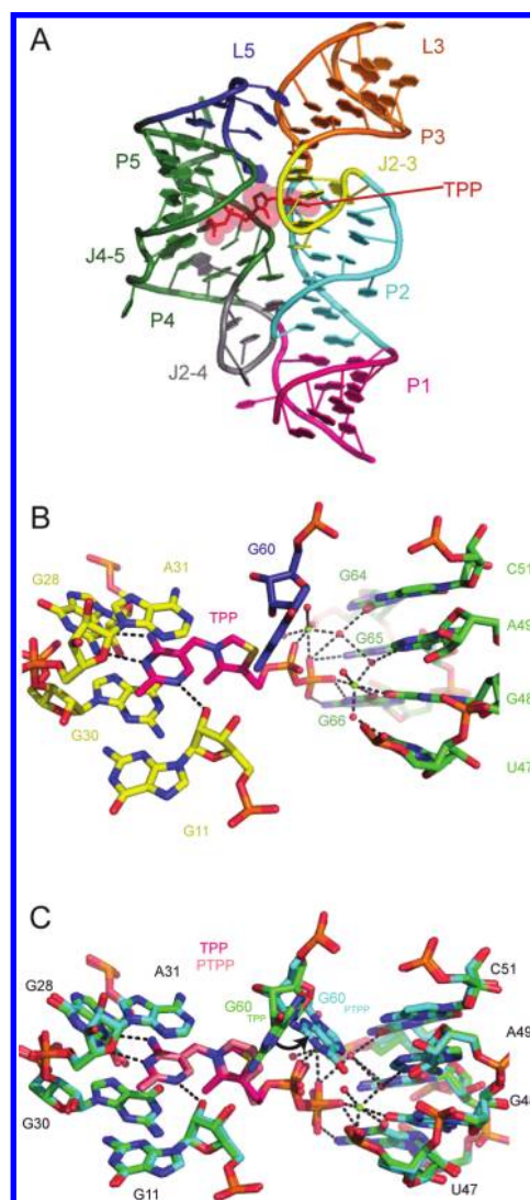
FIGURE 2. (A) The Arabidopsis thaliana TPP riboswitch 39 with TPP (red) bound (PDB 3D2G). (B) Mg^{2+} and waters (green and red spheres, respectively) in the ligand binding site. (C) Superposition of TPP (RNA, green; TPP, magenta) and PTPP (RNA, cyan; PTPP, pink, PDB 3D2V) bound to the RNA. Black arrow denotes movement of G60 between the two structures.
