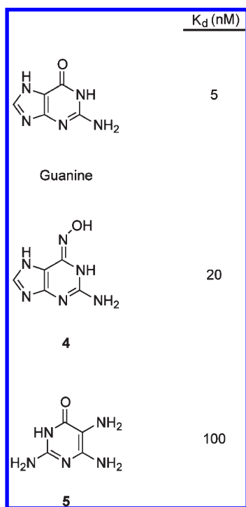
FIGURE 5. Guanine analogs that bind the guanine riboswitch: (Z)-2-amino-1H-purin-6(9H)-one oxime ( 4 ) and 2,5,6-triaminopyrimidin-4-one ( 5 ). K_D values from refs 53 and 54.
