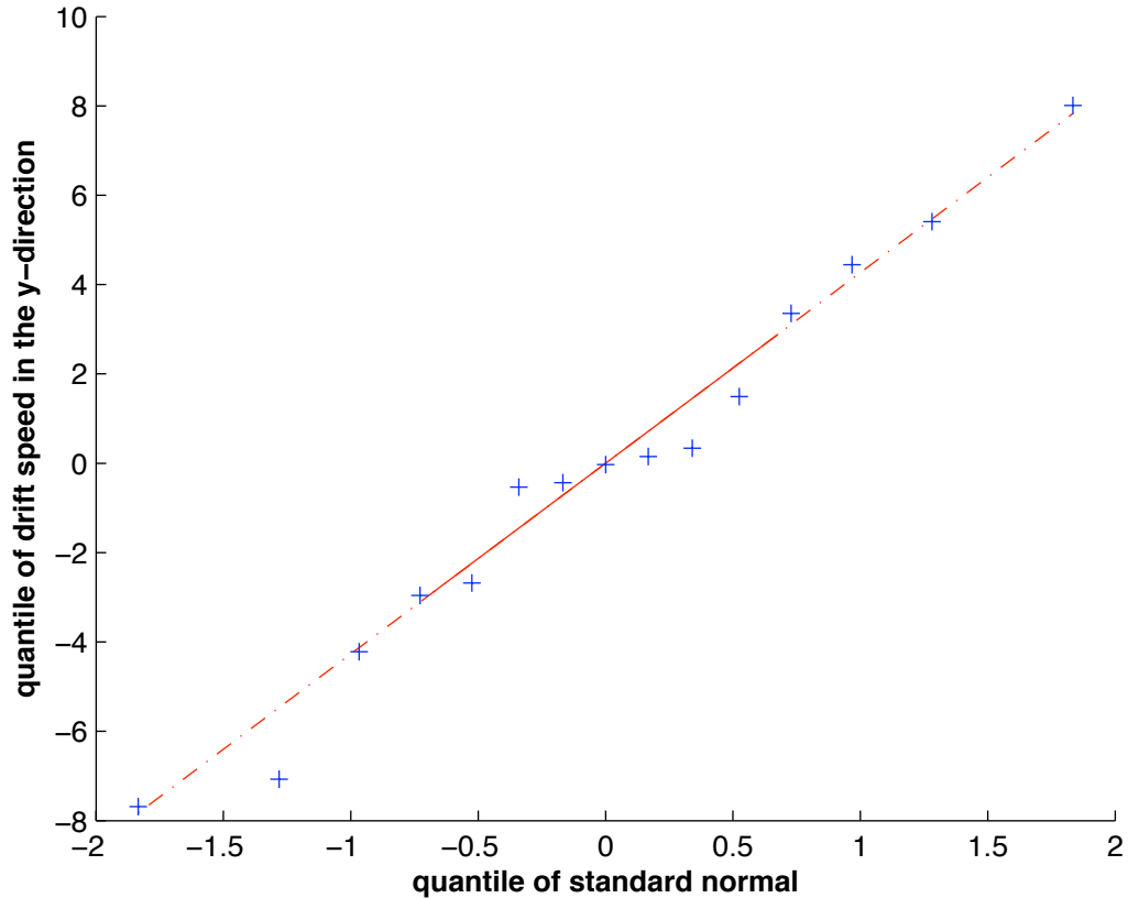
qq-plot to assess the normality of the drift speed in the y direction
