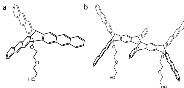
Figure 1. Structure of antrip-DEG and its photodimer.
