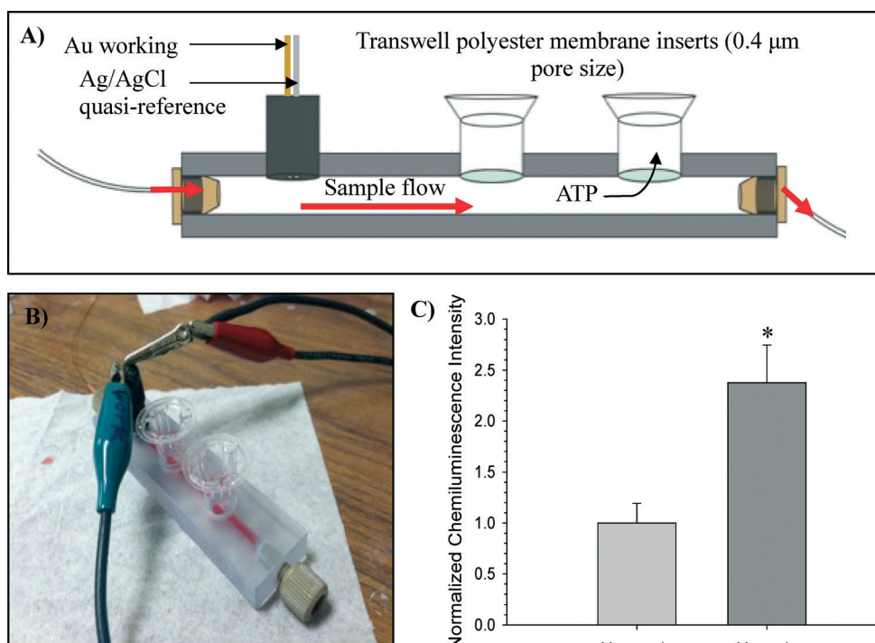
Fig. 6 Fluidic device for correlation of oxygen tension and ATP release. A) Schematic of device; B) picture of the assembled device with RBCs being pumped through the system; C) comparison of RBC ATP release from a normoxic sample ( 8.22 \pm 0.60 ppm oxygen) to a moderately hypoxic sample ( 4.76 \pm 0.53 ppm oxygen). N = 3 donors; error = s.e.m., * p < 0.05 .
