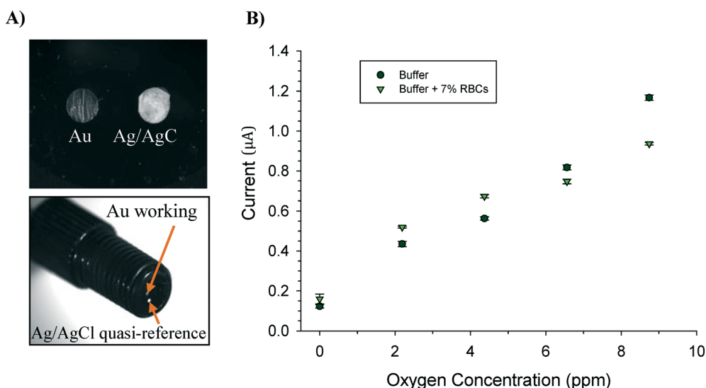
Fig. 4 Measuring \text{O}_2 tension in a flowing stream of buffer (HBSS) and in HBSS with RBCs. Measurements were made with a Nafion-coated gold electrode and Ag/AgCl quasi-reference electrode. A) Micrographs of the electrode containing gold and silver wire secured with C-7 epoxy. In both micrographs, the silver wire is coated with AgCl; B) calibration curve data for oxygen standards in HBSS [ y = 1.13 \times 10^{-7} \times +1.26 \times 10^{-7} ; R^2 = 0.98 ] and in the presence of RBCs [ y = 8.15 \times 10^{-8} \times +2.50 \times 10^{-7} ; R^2 = 0.93 ]. n = 1 electrode with triplicate measurement. Error = standard deviation.
