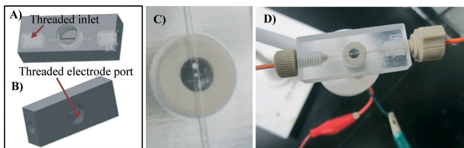
Fig. 1 3D device used for electrochemical detection. A–B) 3D renderings of the device in Autodesk software; C–D) printed 0.5 mm-wide channel device in VeroClear material. The Pt-electrode is screwed into the electrode port, showing alignment of both Pt wires with the 0.5 mm channel (panel C). In panel D, the device is shown with the Pt-electrode, electrode leads, and the fittings used to integrate the device with a syringe pump.
