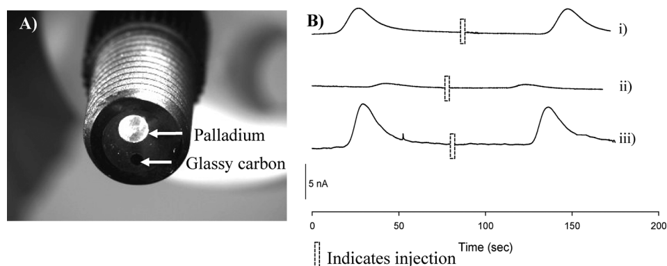
Fig. 2 Glassy carbon working electrode for the detection of dopamine. A) Image showing the flangeless fitting with a 2 mm palladium pseudo-reference and a 1 mm glassy carbon working electrode; B) flow injection analysis to show selectivity of a Nafion-coated glassy carbon electrode; i) response for dopamine [100 \mu\text{M} ] using the Nafion-coated glassy carbon electrode; ii) response for nitrite [100 \mu\text{M} ] using the Nafion-coated glassy carbon electrode; iii) response for nitrite [100 \mu\text{M} ] using a non-modified glassy carbon electrode.
