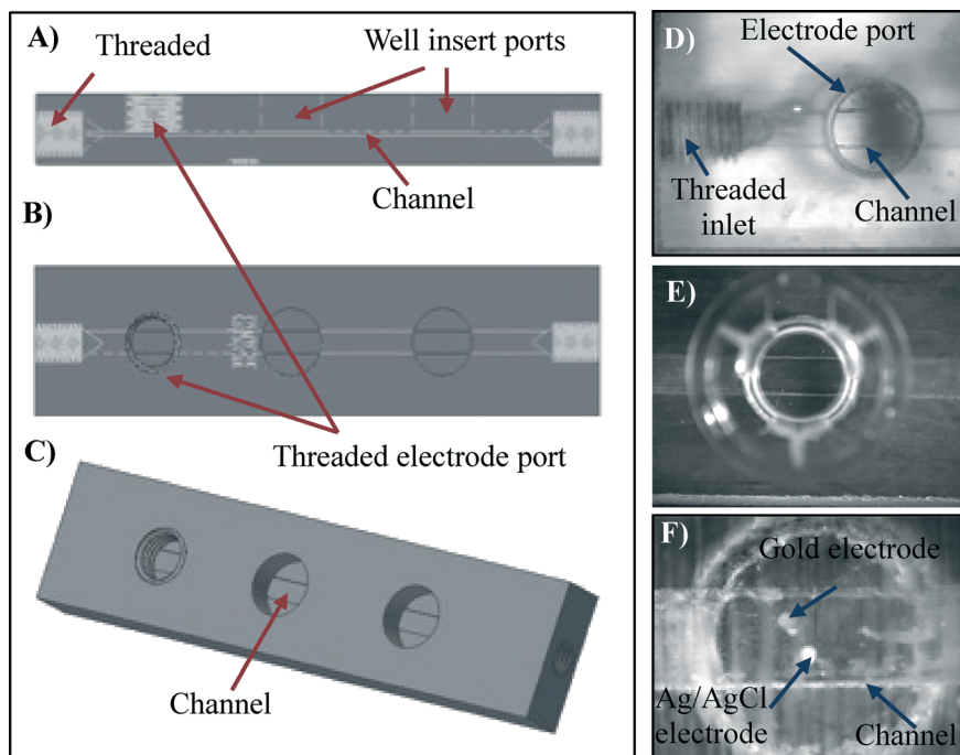
Fig. 5 Fabrication of 3D device to measure oxygen and ATP from flowing RBCs. The left side of the figure shows the rendering of the device in the Autodesk software. A) Side profile of device detailing the threaded inlet, electrode port, and well insert ports; B) top view of device; C) solid body view of device; D) 3D printed device in VeroClear material, detailing the inlet and electrode port; E) transwell membrane inserted into the device via the well insert port; F) 3D printed device with electrode inserted fully into the port, showing the working and quasi-reference electrodes for oxygen sensing.
