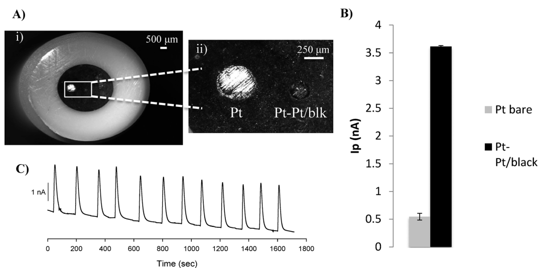
Fig. 3 Platinum electrodes for NO detection. A) i) Platinum pseudo-electrode (500 \mu\text{m} ) and platinum working electrode [250 \mu\text{m} ] encapsulated with epoxy in a flangeless fitting; ii) zoomed micrograph of the platinum black modified platinum working electrode; B) bar graph comparing the signal for NO [190 \mu\text{M} ] with a bare Pt electrode versus the Pt/Pt-black modified electrode; C) amperogram of reproducible 190 \mu\text{M} NO injections over the Pt/Pt-black electrode.
