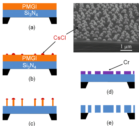
FIG. 1. (Color online) Schematic of porous membrane fabrication process. (a) Spin-coat PMGI film onto \text{Si}_3\text{N}_4 membrane. (b) Thermally evaporate CsCl film and allow it to self-assemble in the presence of moisture. (c) RIE PMGI to obtain undercut profile. (d) Evaporate Cr layer and lift it off. (e) RIE silicon nitride and (optional) remove Cr to form porous membrane.
