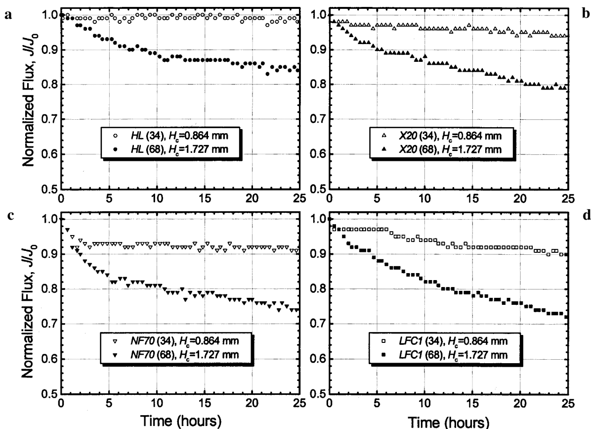
Figure 6. Normalized flux decline data for colloidal fouling experiments conducted with four commercial RO/NF membranes HL (a), X20 (b), NF70 (c), and LFC1 (d). All experiments were conducted at constant physico-chemical conditions of 1.4 \times 10^{-5} m/s (30 gfd) initial flux, 0.01 M NaCl, 200 mg/L (0.08% v/v) 100 nm silica colloids, 25°C, and pH 6.8 \pm 0.2 . A constant feed flow rate of 0.95 Lpm provided shear rates of 1336 \text{ s}^{-1} and 334 \text{ s}^{-1} in the 34 unit ( H_c = 0.864 mm) and the 68 unit ( H_c = 1.73 mm), respectively.
