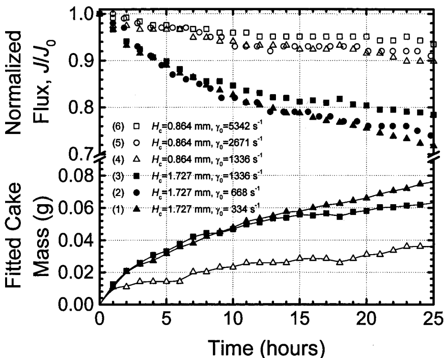
Figure 7. Normalized flux decline and fitted cake mass data for reverse osmosis membrane LFC1 in CMF units with different channel height over a range of feed flow rates, crossflow velocities, and shear rates. All runs in the thin-channelled 34 unit ( H_c = 0.864 \text{ mm} ) exhibit less flux decline than those in the 68 unit ( H_c = 1.73 \text{ mm} ). Other experimental conditions are as in Fig. 6.
