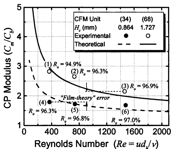
Figure 4. Comparison of theoretical and experimental concentration polarization (CP) modulus ( C_m/C_b ) vs. Reynolds number for the lab-scale CMF units. The numbers in parentheses correspond to the item numbers in Table 1. According to the “film-theory” predictions, the CP modulus should be the same for experiments 3 and 4. Both predicted and experimental CP modulus values were determined at J_0 = 1.42 \times 10^{-5} m/s (30 gfd), C_b = 0.01 M NaCl, pH = 6.8 \pm 0.2 , and 25^\circ\text{C} .
