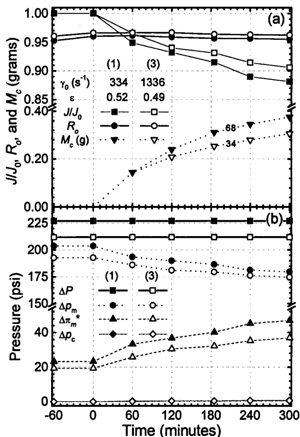
Figure 9. Data for LFC1 from experiments 1 and 3 (Fig. 7) in the 68 unit, conducted at constant physico-chemical conditions of 1.4 \times 10^{-5} \text{ m/s} (30 gfd) initial flux, 0.01 M NaCl, 200 mg/L (0.08% v/v) 100 nm silica colloids, 25^\circ\text{C} , and \text{pH } 6.8 \pm 0.2 . The feed flow rates were 0.95 and 3.8 Lpm resulting in wall shear rates of 334 and 1336 \text{ s}^{-1} , respectively. In (a) measured values of normalized flux decline ( J/J_0 ), observed salt rejection ( R_o ), and cake layer mass ( M_c ) are plotted against time of filtration. In (b) applied pressure ( \Delta P ), trans-membrane pressure ( \Delta p_m ), cake-enhanced osmotic pressure ( \Delta \pi_m^* ), and trans-cake pressure ( \Delta p_c ) are plotted against time of filtration.
