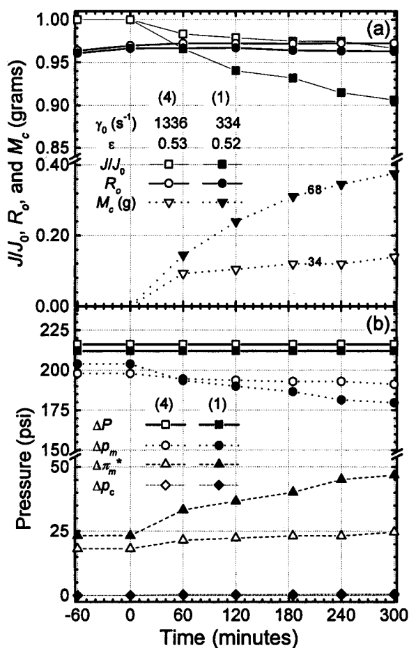
Figure 8. Data for LFC1 from experiments 1 and 4 (Fig. 7) in the 68 and 34 units, respectively, conducted at constant physico-chemical conditions of 1.4 \times 10^{-5} \text{ m/s} (30 gfd) initial flux, 0.01 M NaCl, 200 mg/L (0.08% v/v) 100 nm silica colloids, 25^\circ\text{C} , and \text{pH } 6.8 \pm 0.2 . The feed-flow rate was 0.95 Lpm in both filters resulting in wall shear rates of 334 and 1336 \text{ s}^{-1} in the 68 and 34 units, respectively. In (a) measured values of normalized flux decline ( J/J_0 ), observed salt rejection ( R_o ), and deposit layer mass ( M_c in grams) are plotted against time of filtration. Cake layer mass, M_c , comes from multiplying the deposit layer mass per unit membrane area, M_d , by the membrane area ( 0.01387 \text{ m}^2 ). In (b) applied pressure ( \Delta P ), trans-membrane pressure ( \Delta p_m ), cake-enhanced osmotic pressure ( \Delta \pi_m^* ), and trans-cake pressure ( \Delta p_c ) are plotted against time of filtration.
