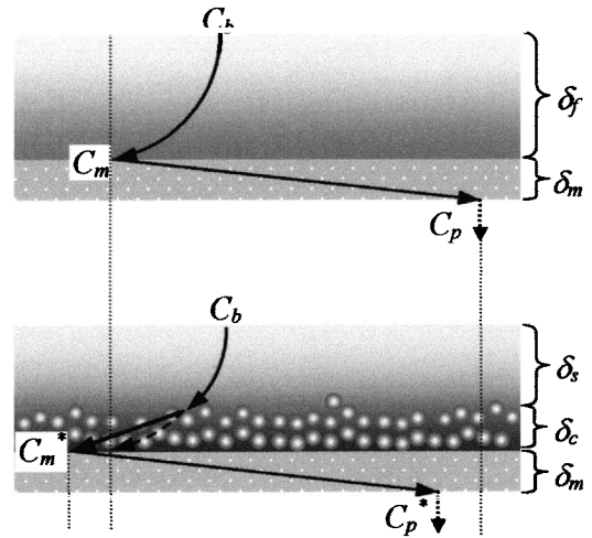
Figure 1. Conceptual illustration of “cake-enhanced osmotic pressure” effect. In the absence of a colloid deposit layer (top figure), the elevated concentration at the membrane surface ( C_m ) decays to the bulk concentration ( C_b ) over the salt concentration polarization (film) layer thickness ( \delta_f ). The salt concentration drops across the membrane thickness ( \delta_m ) due to salt rejection. For a thin deposit layer (bottom figure), the film layer thickness remains constant and the difference between \delta_f and cake thickness ( \delta_c ) is \delta_s . In the presence of a colloid deposit layer the membrane surface salt concentration is enhanced ( C_m^* ) due to hindered back-diffusion of salt ions and a decrease in salt rejection results. The elevated C_m^* will also result in elevated permeate salt concentration, C_p^* .
