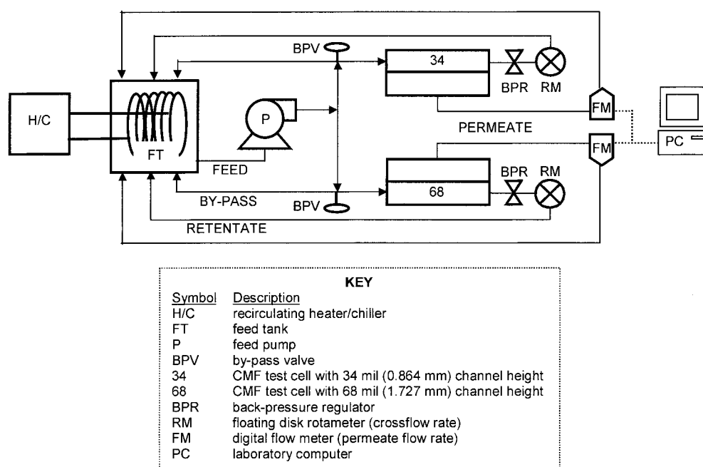
Figure 3. Crossflow membrane filtration (CMF) apparatus used in experiments designed to simultaneously test the influence of crossflow hydrodynamics and membrane filter geometry on colloidal fouling. The two crossflow membrane filters may be fed in parallel from a common feed tank, or individually.
