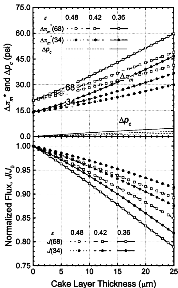
Figure 5. Plot of calculated cake-enhanced osmotic pressure ( \Delta\pi_m^* ) and trans -cake pressure ( \Delta p_c ) as a function of cake layer thickness for several porosities. Mass transfer related effects are simulated using the hydrodynamic conditions described in items (1) and (4) in Table 1. The following parameters used in the calculations: J_0 = 1.42 \times 10^{-5} m/s (30 gfd), R_m = 10^{-11} Pa-s/m; \Delta P_{34} = 220 psi and \Delta P_{68} = 227 psi; Q = 0.95 Lpm; \gamma_{0,34} = 1336 \text{ s}^{-1} and \gamma_{0,68} = 334 \text{ s}^{-1} ; C_b = 0.01 M NaCl; and 0.97 \geq R_{o,34} \geq 0.96 and 0.96 \geq R_{o,68} \geq 0.95 .
